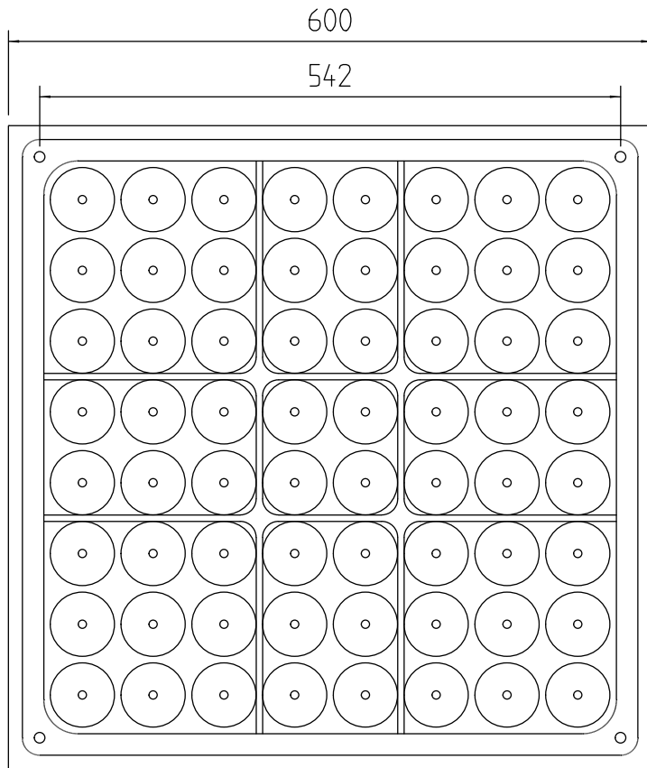
Bottom View
